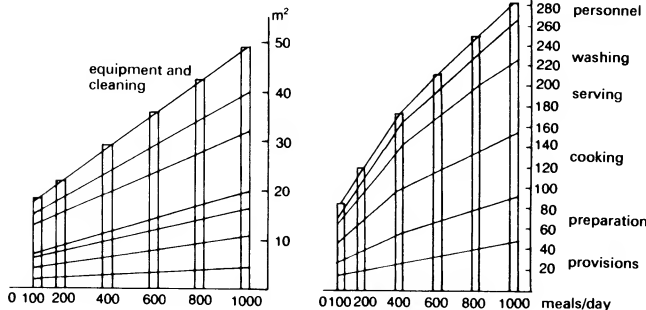
⑨ Meals/day: base kitchen size in m 2 ⑩ Meals/day: areas for different service types
